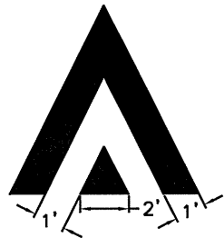
PAVEMENT MARKING DETAIL
