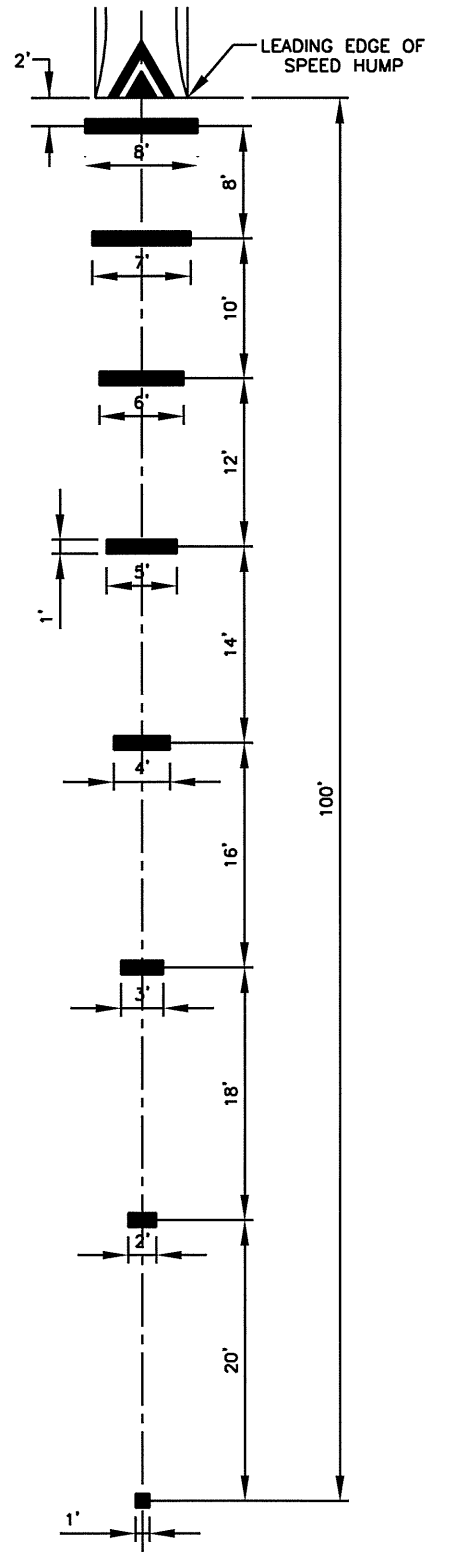
SPEED HUMP ADVANCE WARNING MARKINGS
