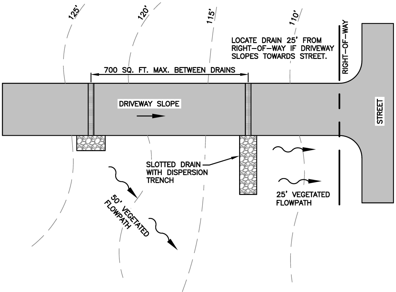
STEEP DRIVEWAY WITH SLOTTED DRAINS
