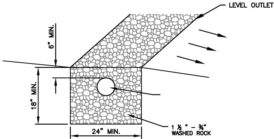
TRENCH CROSS-SECTION
